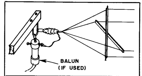
Fig. 3 — Center-support and end-taper detail of the cage.
